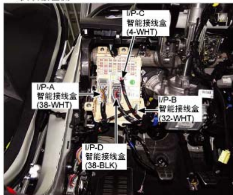
76.仪表板左侧
